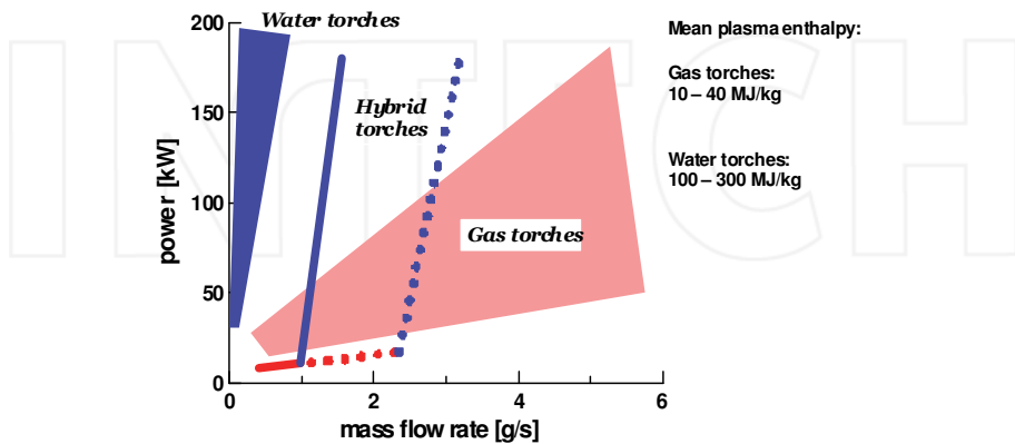
Fig. 13. Operation regimes of dc arc plasma torches.
